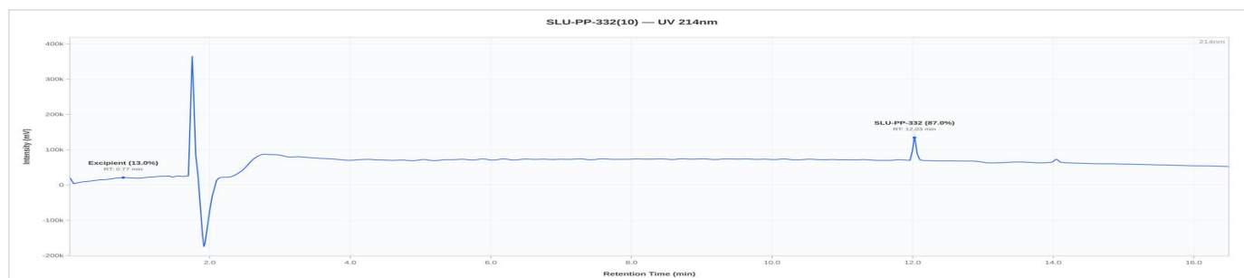
SLU-PP-332 10 - S32798: UV Chromatogram
