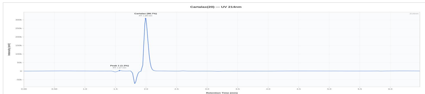
Cartalax 20 - C64953: UV Chromatogram
