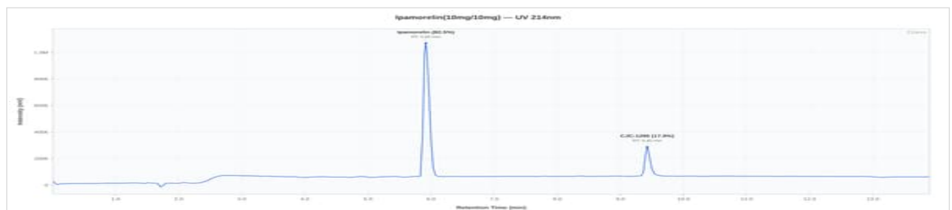
CJC 1295 No DAC / Ipamorelin Blend 10mg/10mg - C31965: UV Chromatogram
