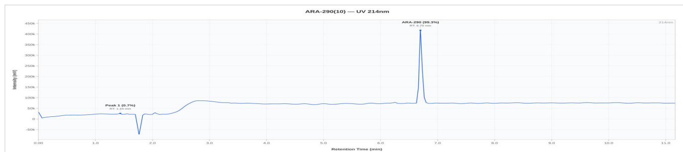
ARA-290 10 - A63981: UV Chromatogram
