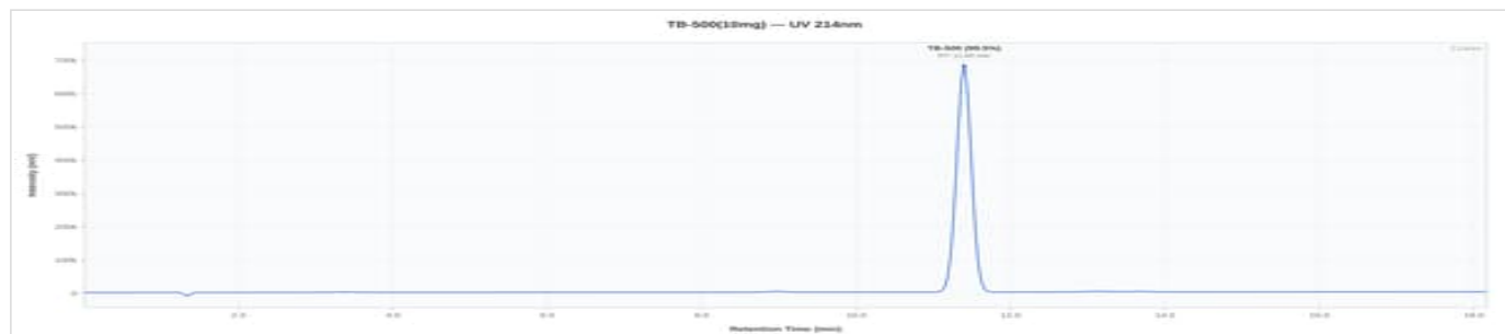
TB-500 10mg - T68194: UV Chromatogram
